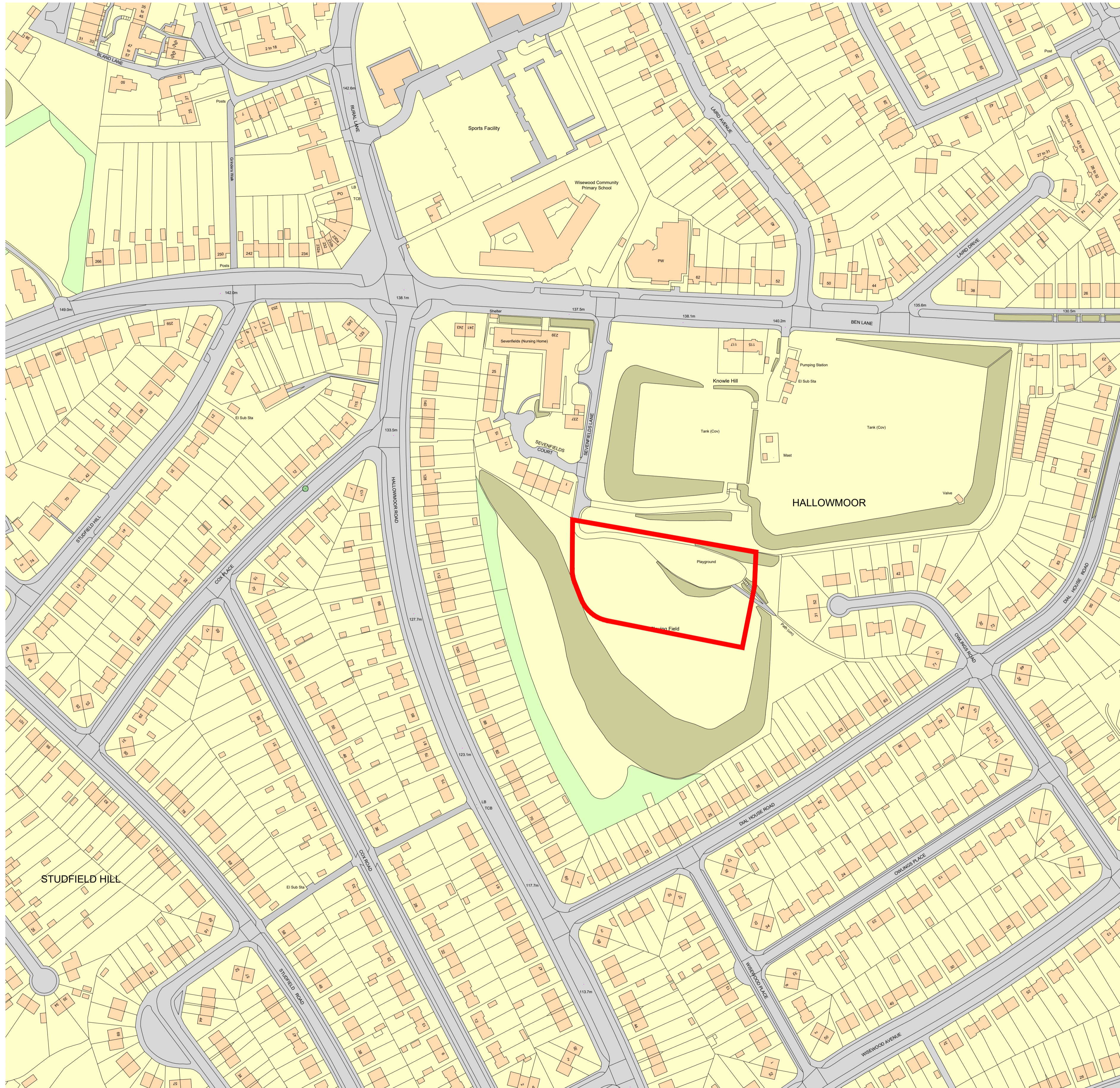
LOCATION PLAN 1:1250
